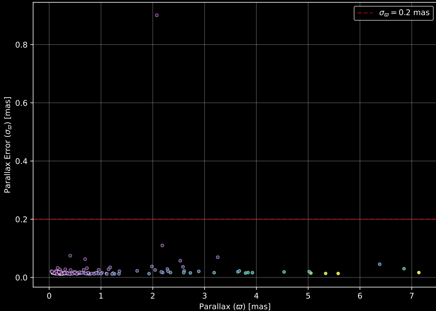
APOGEE DR17 Field: [N2204] Parallax Quality (n= 175)
