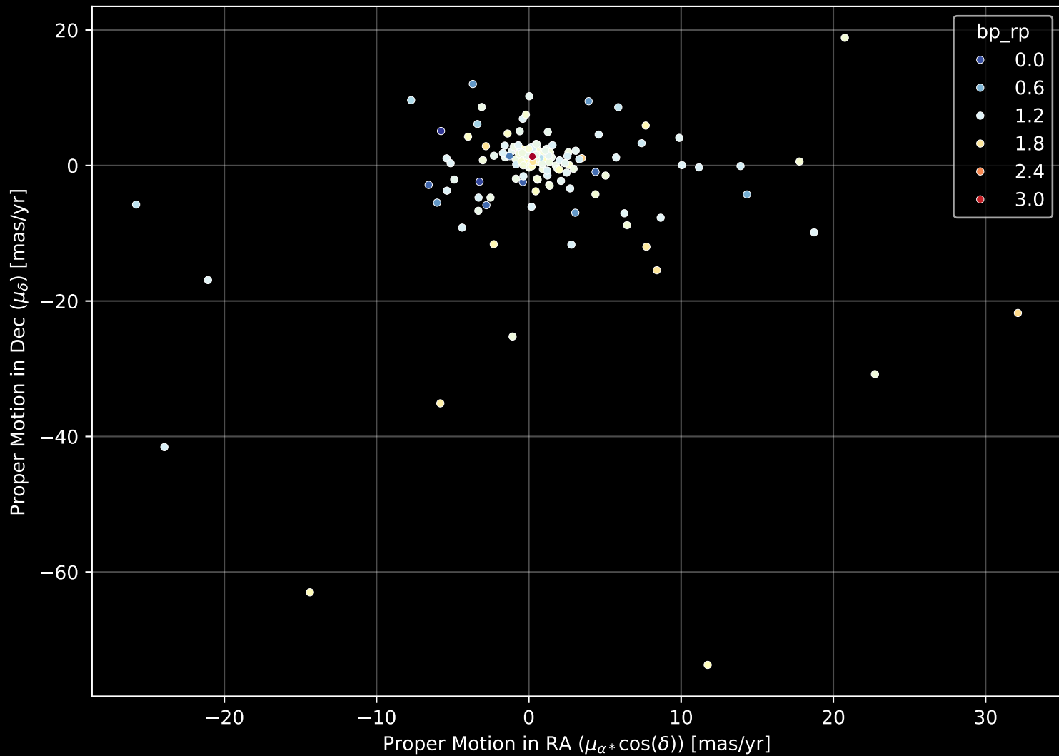
APOGEE DR17 Field: [N2204] Proper Motion Diagram (n= 175)
