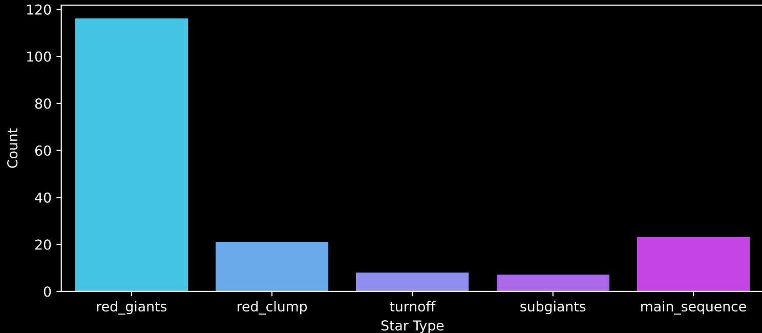
APOGEE DR17 Field: [N2204] Count plot of Star Type
