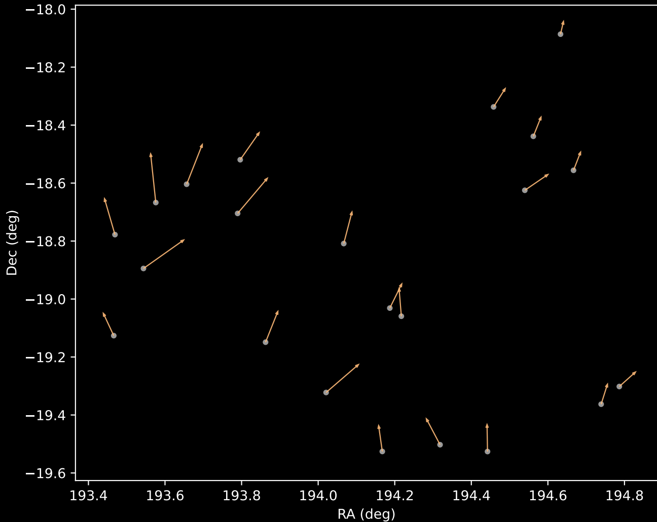
APOGEE DR17 Cluster 3 Proper Motion Vectors (n=22)
