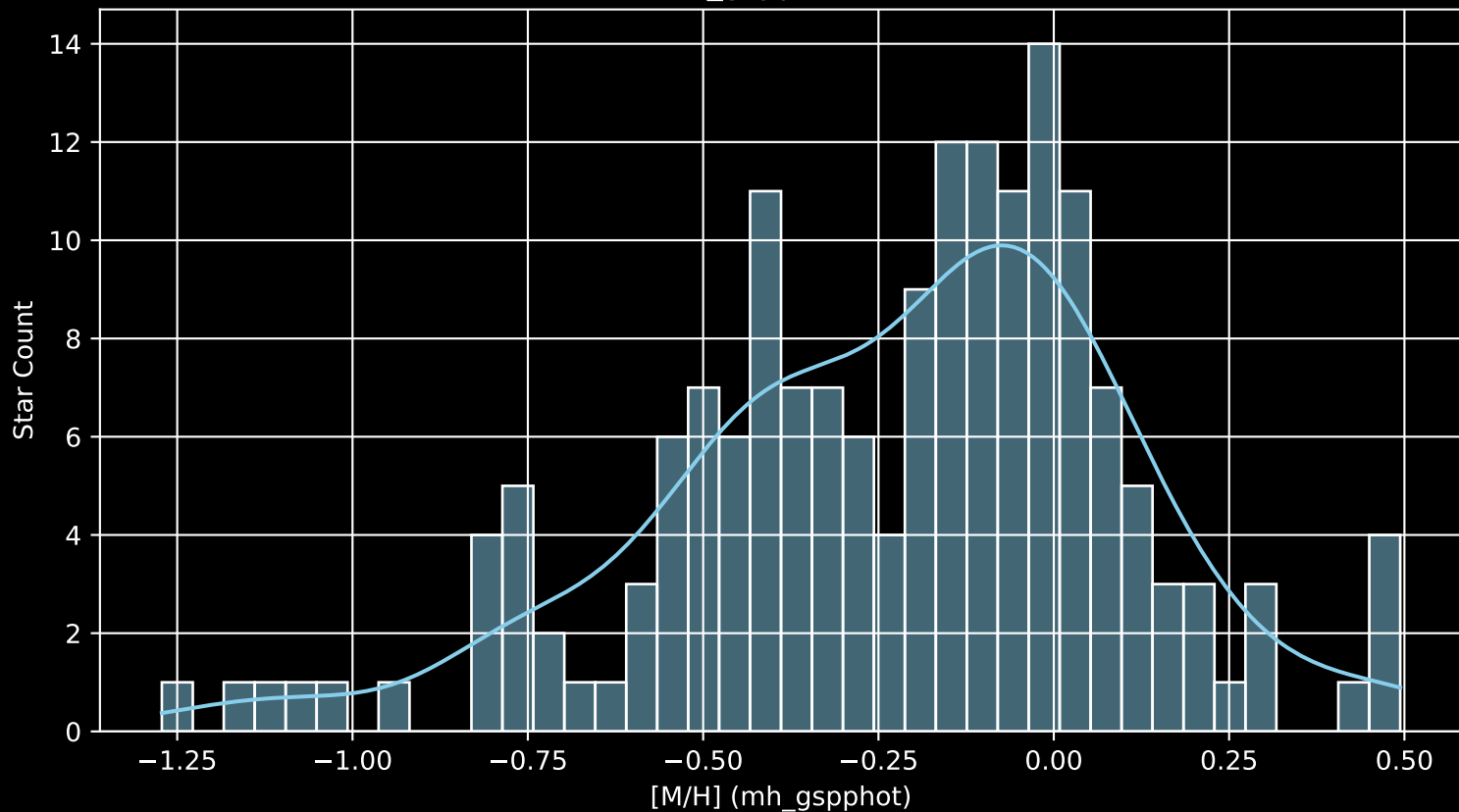
APOGEE DR17 Field: [N2204 [M/H] (mh_gspphot) (n= 172)
