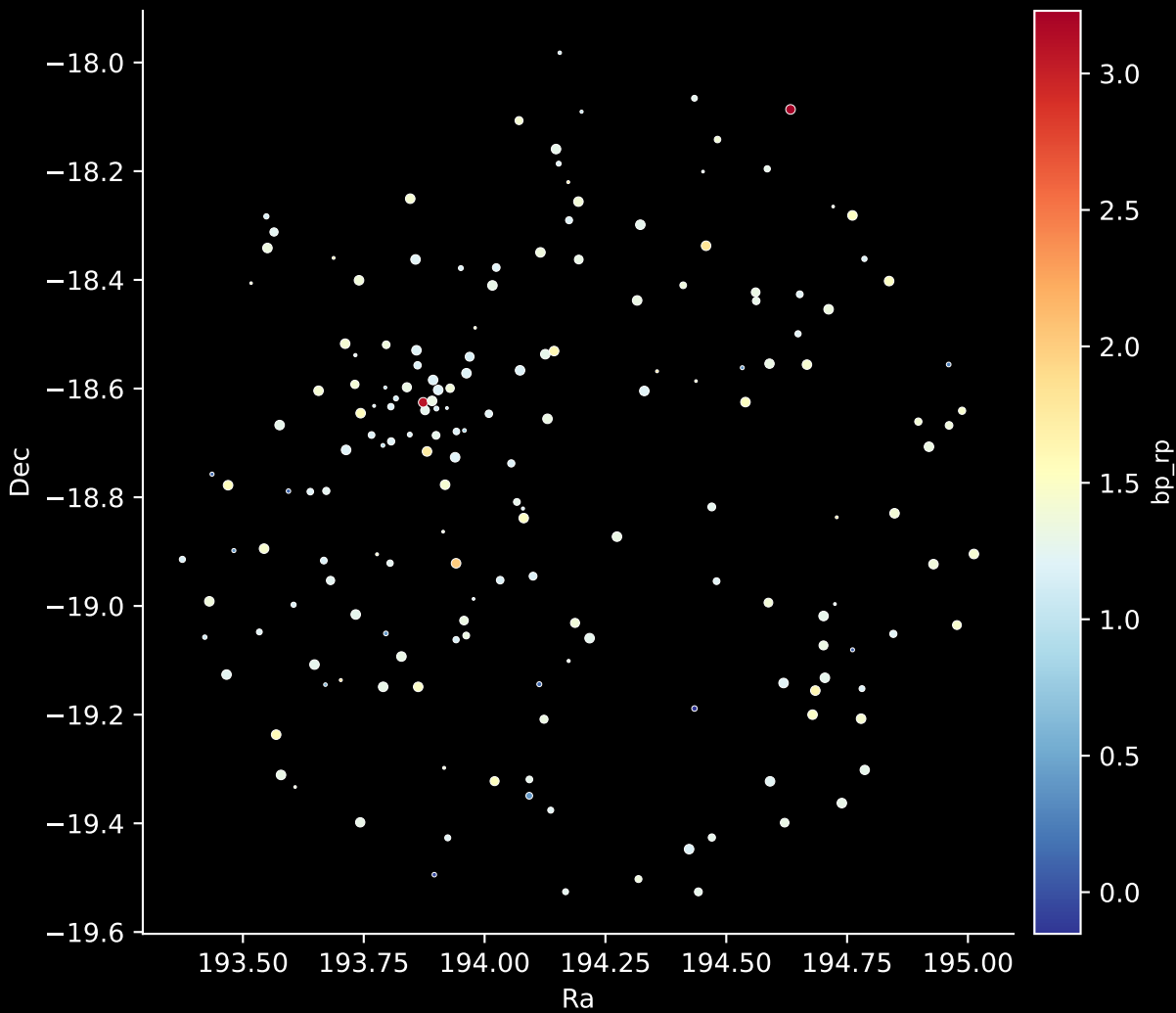
APOGEE DR17 Field: [N2204] Stars: 175
