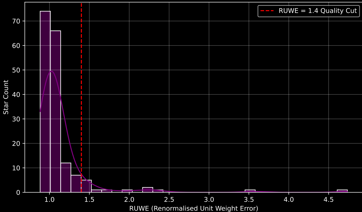
GAPOGEE DR17 Field [N2204] RUWE Distribution (n= 172)
